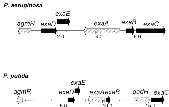
Fig. 1 The agmR – exa gene cluster of Pseudomonas aeruginosa (constructed from sequence data; GenBank accession no. AJ009858) and the agmR – exa cluster of P. putida (constructed from KT2440 sequence data at http://www.tigr.org ). Genes encode: exaD sensor kinase, exaE response regulator, exaA quinoprotein ethanol dehydrogenase, exaB cytochrome c precursor, qadH uncharacterized pyrroloquinoline quinone (PQQ)-linked alcohol dehydrogenase detected from P. putida KT2440 genome sequence data, exaC aldehyde dehydrogenase. Scale markings represent DNA length in kilobases
